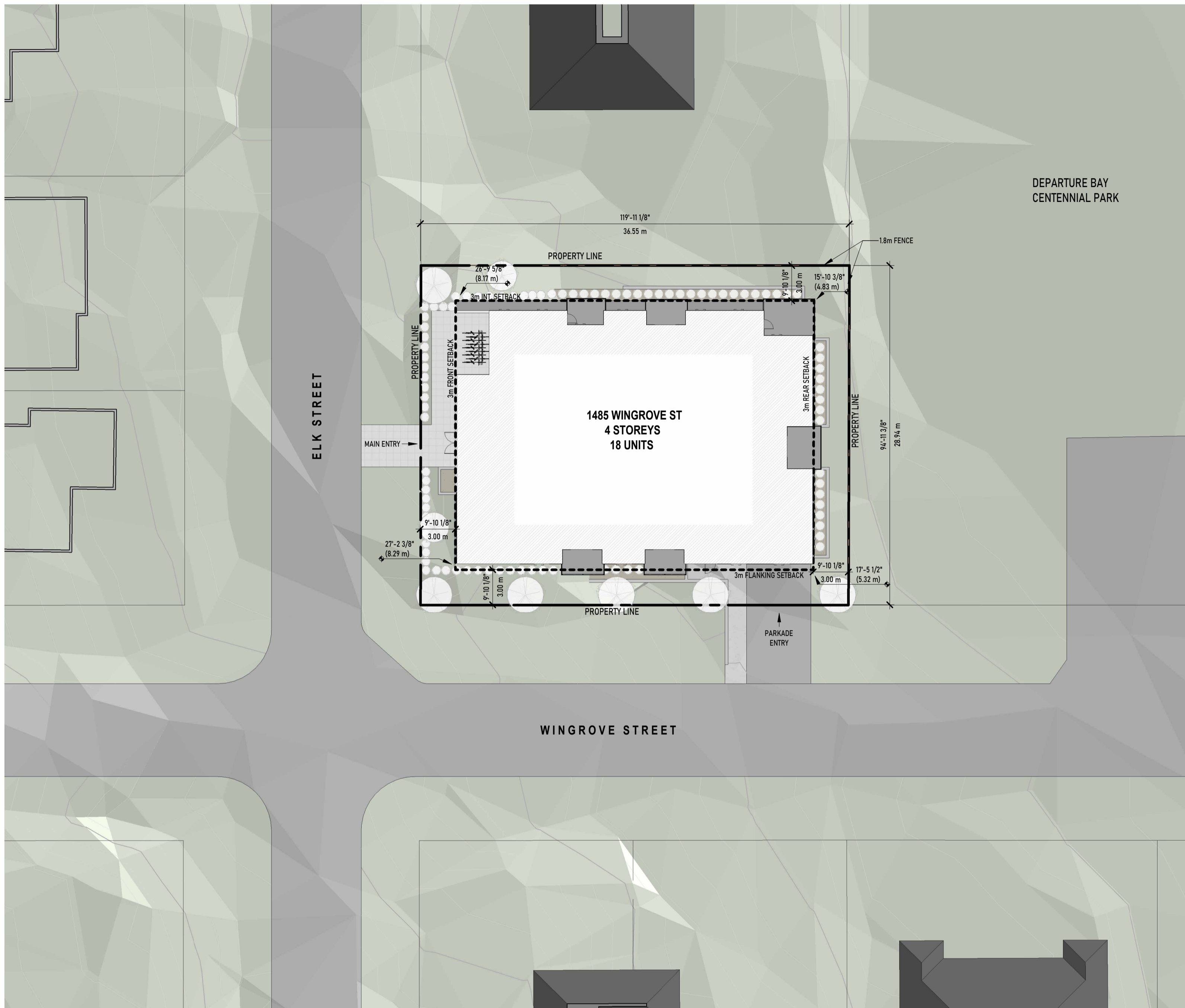
5 SITE PLAN SD1 1" = 20'-0"
